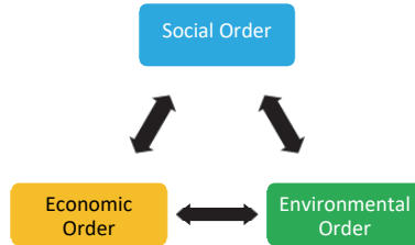
Fig. 1. Interactions in three main areas of Integrated Order
