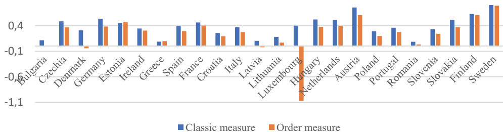
Fig. 2. Values of classic and order synthetic measure according to integrated order
