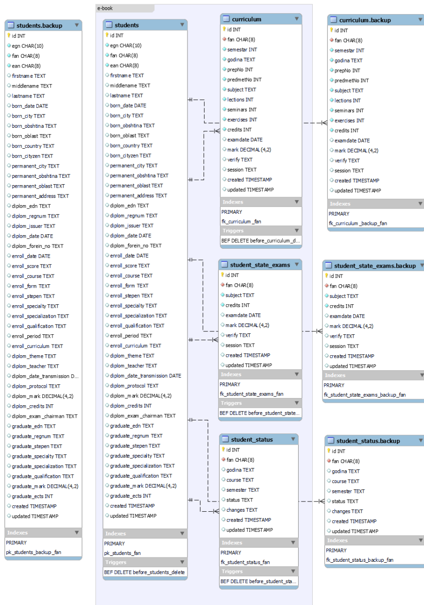
Фиг. 4. Entity Relationship (ER) Diagram
